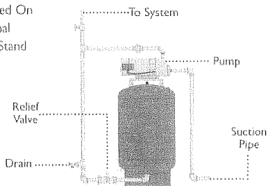
FLEXCON TANK WITH JET PUMP
