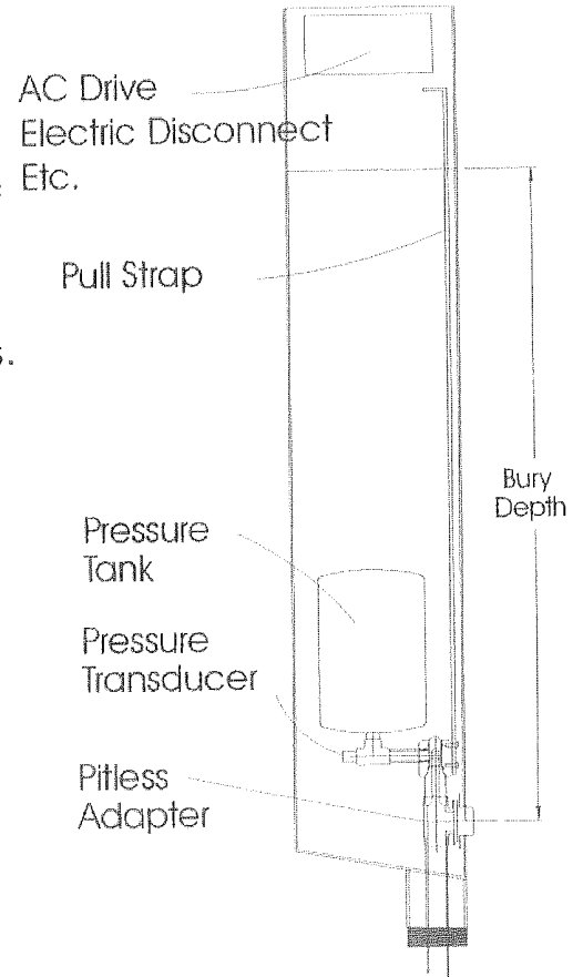
PCM for Variable Speed Pump
