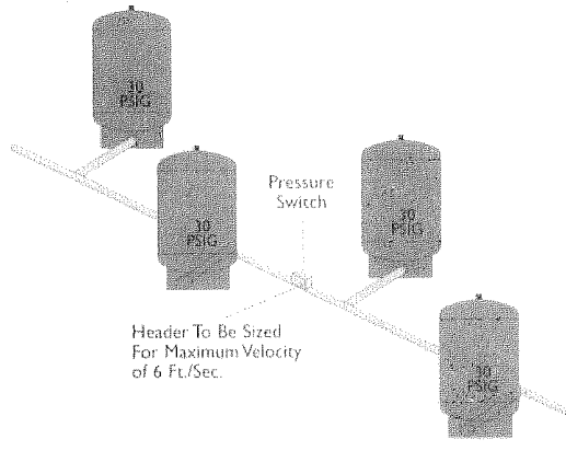
FLEXCON MULTI-TANK INSTALLATION - OPTION B
