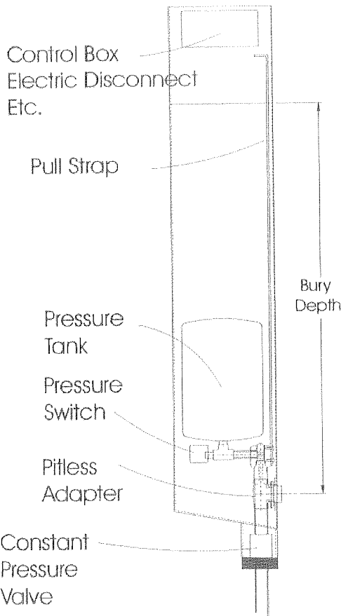
PCM for Constant Speed Pump
