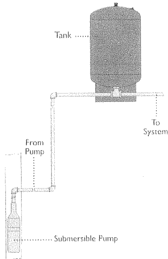
FLEXCON TANK WITH SUBMERSIBLE PUMP
