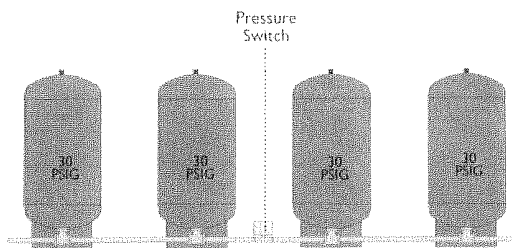
FLEXCON MULTI-TANK INSTALLATION - OPTION A
